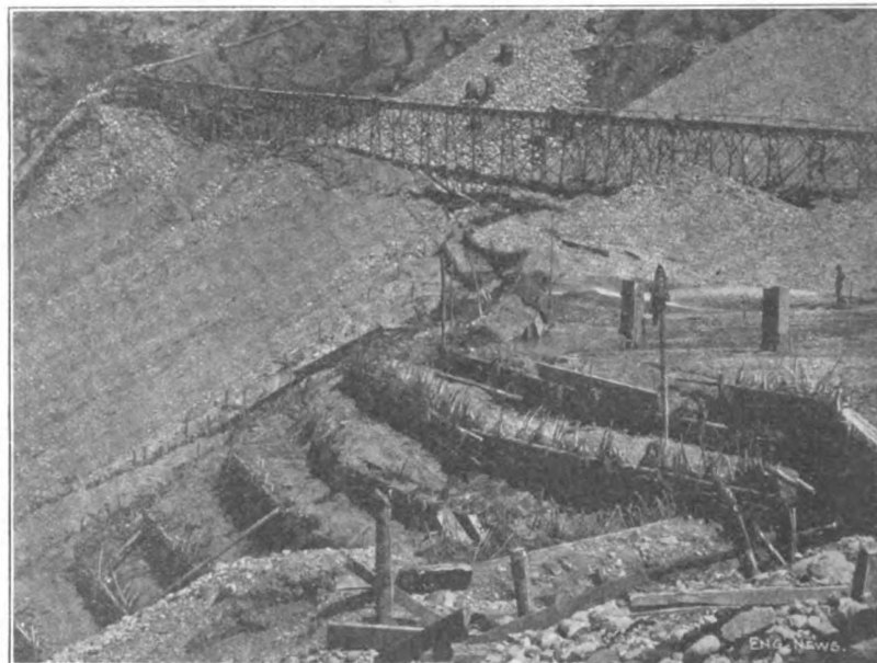
FIG. 9. BRUSH AND POLE DIKES FOR BUILDING UP THE SLOPE OF THE BANK.
