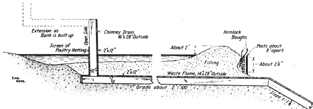
FIG. 7. ARRANGEMENT OF BOX DRAINS AND "CHIMNEYS" FOR CARRYING OFF WATER FROM SETTLING POOL ON TOP OF HYDRAULIC-FILL BANK.
